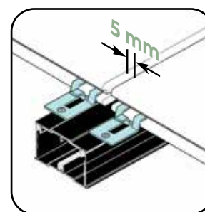
Silvadec® aluminium joist + single fastening clips
